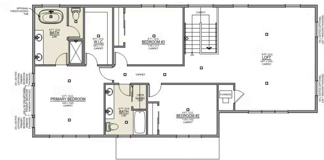
UPPER FLOOR
