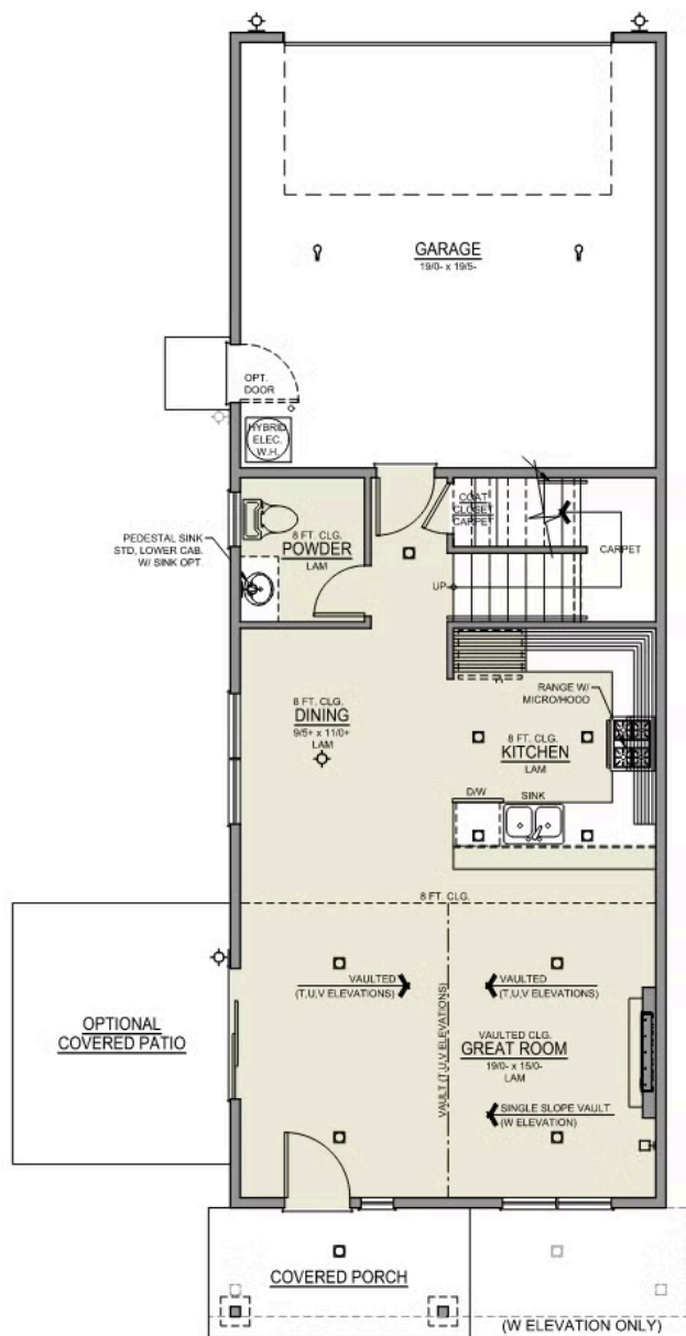
MAIN FLOOR
