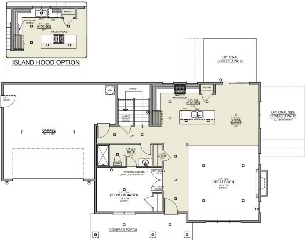
MAIN FLOOR
