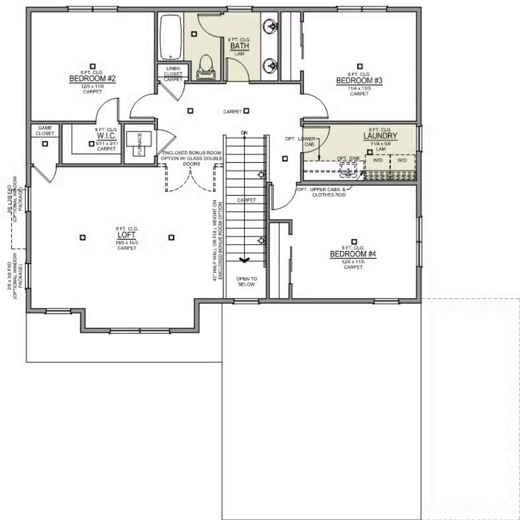
UPPER FLOOR
