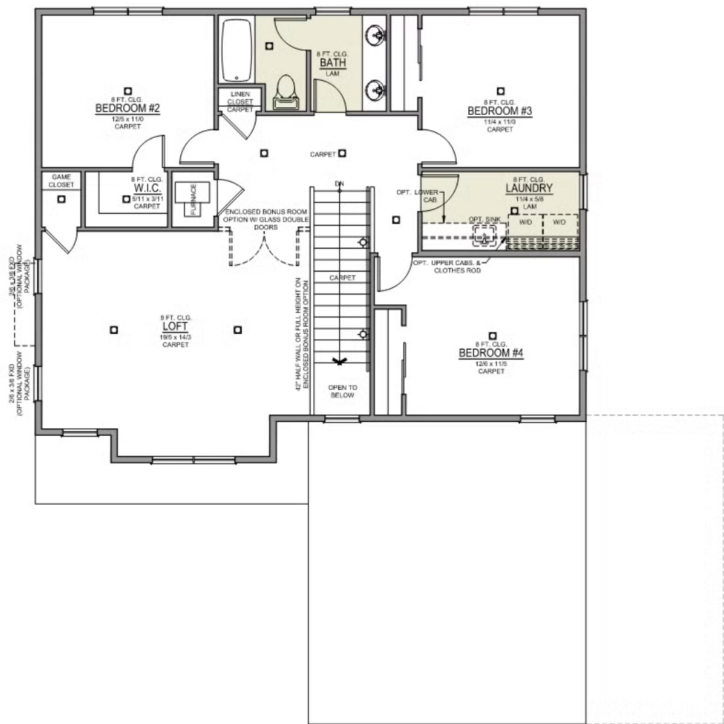
UPPER FLOOR
